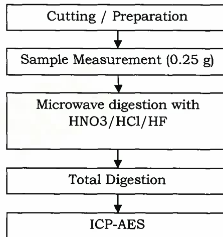
Flow Chart of Digestion for Plastic –EPA3052 for Pb、Cd (without residue)
